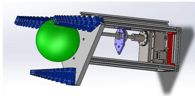
FIGURE III.10 – Assemblage de notre pince
