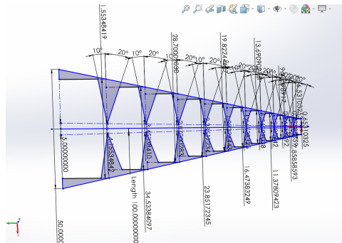
FIGURE III.7 – Ligne de construction
