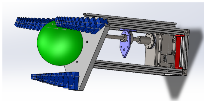
FIGURE III.10 – Accouplement de notre pince
