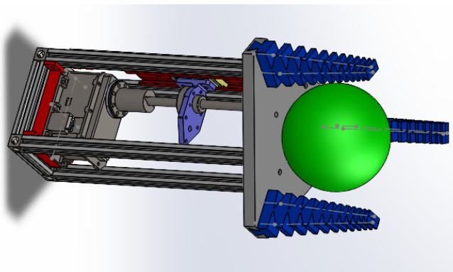
FIGURE III.10 – Assemblage de notre pince
