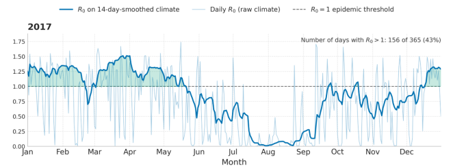
Figure 3: Seasonal variation of the basic reproduction number R_0 for the calibrated model in 2017.
