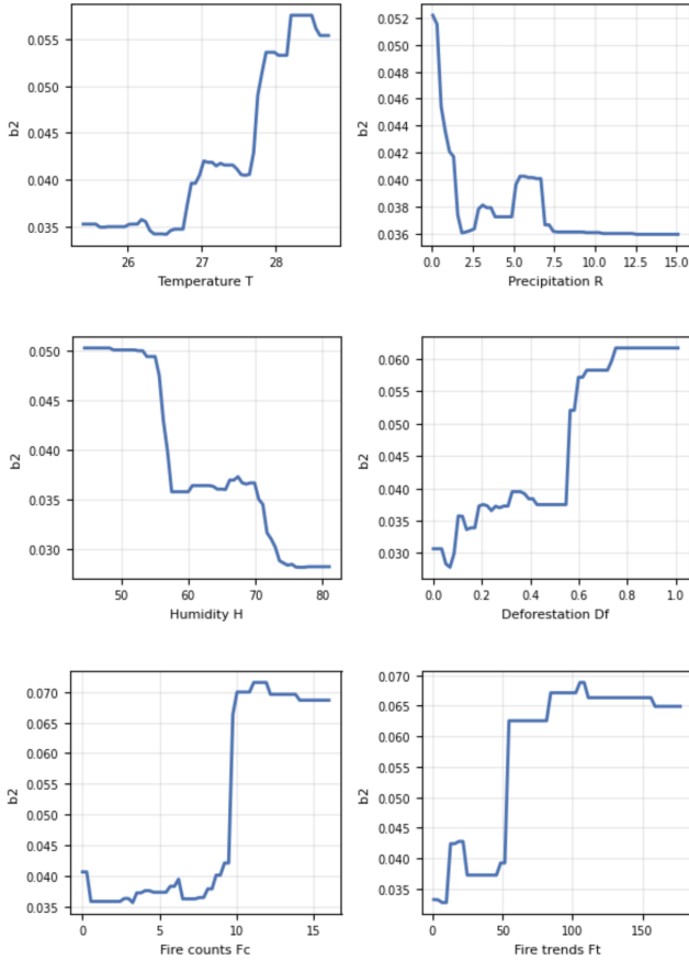
Figure 7: Partial dependence of the weekly per-bite transmission probability b_2 on each environmental predictor in 2020.
