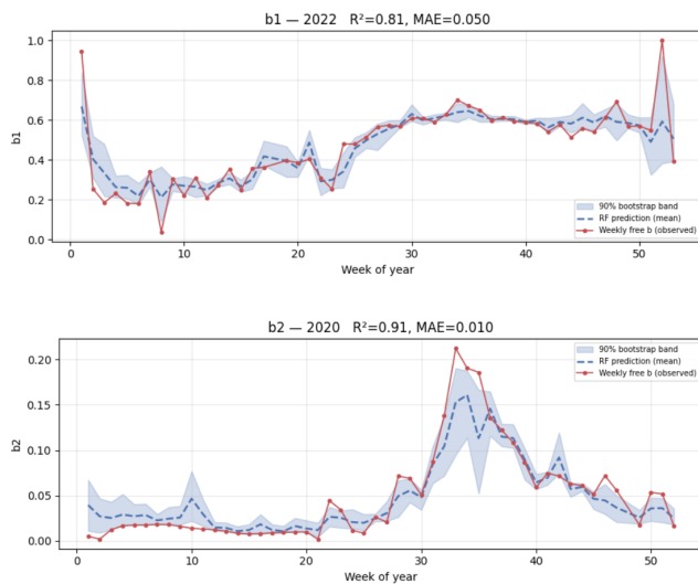
Figure 5: Best within-year random-forest fit of the freed weekly per-bite transmission: 2022 for b_1 ( R^2 = 0.81 ) and 2020 for b_2 ( R^2 = 0.915 ).
