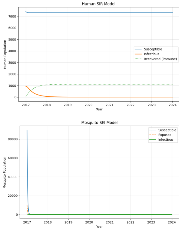
Figure 1A: DDE simulation of the baseline SIR-SEI model using the original parameterization from [16]. The dynamics of the SIR model show a monotonic decline in the number of infected individuals within the human population, indicating the absence of sustained transmission, while the dynamics of the SEI model show that the entire mosquito population tends to extinction, an unexpected behavior for a region where malaria is highly endemic.
