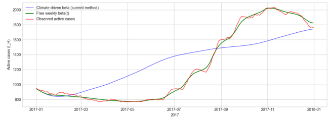
Figure 2: Comparison between the observed active cases and the model estimation of the infectious human compartment I_H for 2017.
