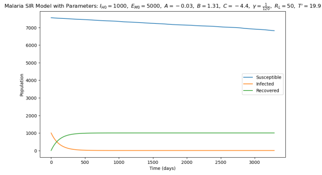
Figure 1A: Results of the initial SIR model, with equations and parameters from [7].
