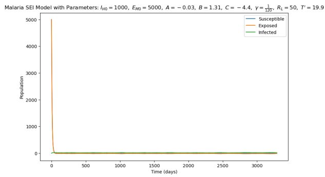
Figure 2A: Results of the initial SEI model, with equations and parameters from [7].
