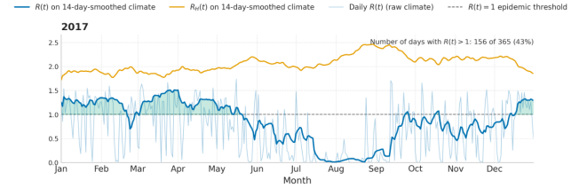
Figure 4: Seasonal variation of the coupled and human basic reproduction number \mathcal{R}(t) for the calibrated model in 2017.
