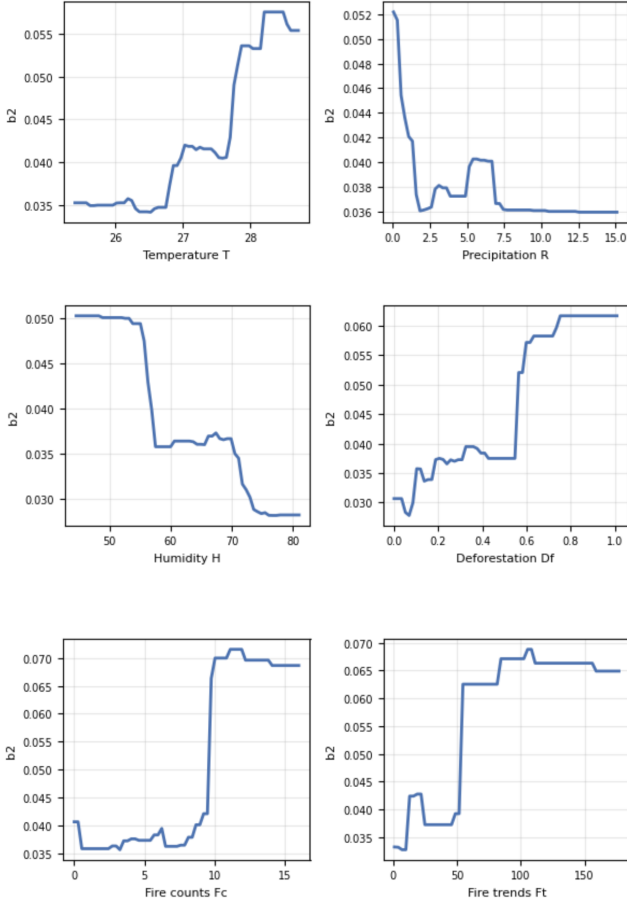
Figure 9: Partial dependence of the weekly per-bite transmission probability b_2 on each environmental predictor in 2020.
