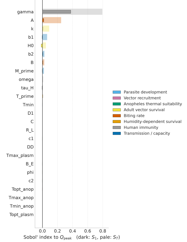
Figure 6: First-order ( S_1 , dark bars) and total-order ( S_T , pale bars) Sobol' indices of the 25 decomposed parameters with respect to the seasonal peak Q_{\text{peak}} of the infectious-human compartment, over the whole admissible parameter box of Table A.3 (Saltelli design, N = 512 ; bars coloured by parameter group). The total-order index also collects the variance that a parameter carries through its interactions with the remaining ones, hence S_T \geq S_1 . Since Q_{\text{peak}} is a maximum, the 74.4% of the sampled parameter sets that are locally subcritical leave it at the initial value I_H(0) ; the indices therefore characterize the sampled box and not the height of an established endemic wave.
