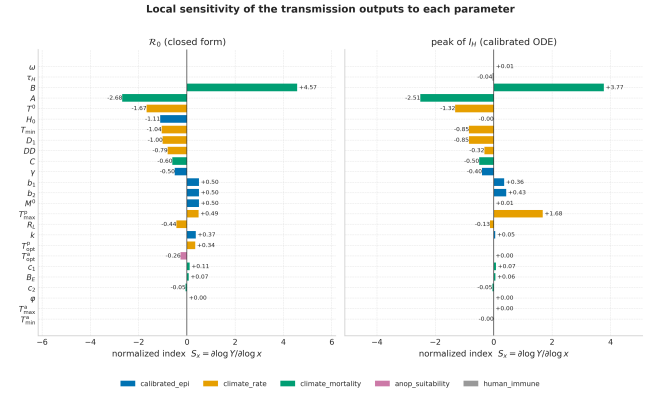
Figure 5: Normalized sensitivity index S_x = \partial \log Y / \partial \log x of the 25 decomposed parameters (bars coloured by parameter group, as in Table 3). Left: closed-form reproduction number at the reference environmental state, by central differences with h = 0.05 ; the exact analytic values of Table 3 differ from these by at most 0.06, the truncation error of the difference quotient. Right: seasonal maximum of the infectious-human compartment of the calibrated model, averaged over 2017-2023, same scheme. A positive index means the output increases with the parameter. The three Anopheles suitability temperatures are exactly zero on the left because the thermal-suitability factor f_T is saturated at the reference climate.
