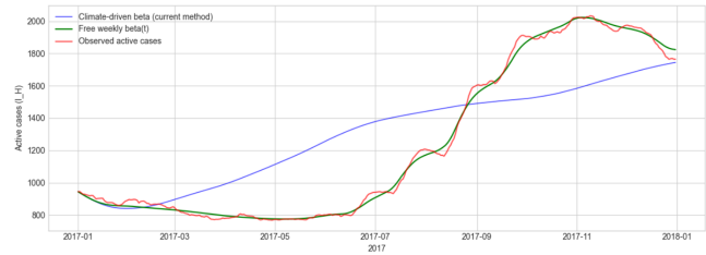
Figure 2: Comparison between the observed active cases and the model estimation of the infectious human compartment I_H for 2017.
