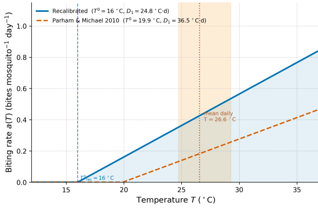
Figure 2: Comparison between the recalibrated temperature-dependent biting rate a(T) used in this work ( T' = 16^\circ\text{C} , D_1 = 24.8^\circ\text{C}\cdot\text{d} ) and the original Parham & Michael (2010) parameterization [11] ( T' = 19.9^\circ\text{C} , D_1 = 36.5^\circ\text{C}\cdot\text{d} ). The shaded band indicates the range of daily mean temperatures observed in Manaus between 2017 and 2023 (5th-95th percentiles), and the dashed vertical line marks the recalibrated biting threshold T' = 16^\circ\text{C} .
