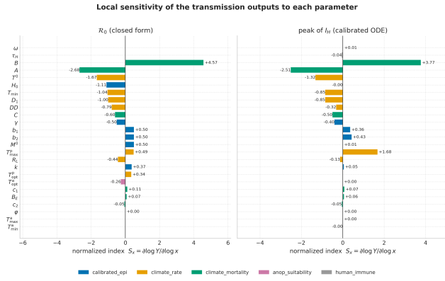
Figure 5: Normalized sensitivity index S_x = \partial \log Y / \partial \log x of the 25 model parameters (bars coloured by parameter group). Left: closed-form reproduction number at the reference environmental state, by central differences with h = 0.05 ; the exact analytic values of Table 3 differ from these by at most 0.06, the truncation error of the difference quotient. Right: seasonal maximum of the infectious-human compartment of the calibrated model, averaged over 2017-2023, same scheme. A positive index means the output increases with the parameter. The three Anopheles suitability temperatures are exactly zero on the left because the thermal-suitability factor f_T is saturated at the reference climate.
