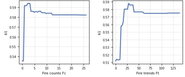
Figure 8: Partial dependence of the weekly per-bite transmission probability b_1 on each environmental predictor in 2022.
