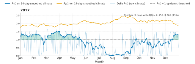
Figure 4: Seasonal variation of the coupled and human basic reproduction number \mathcal{R}(t) for the calibrated model in 2017.
