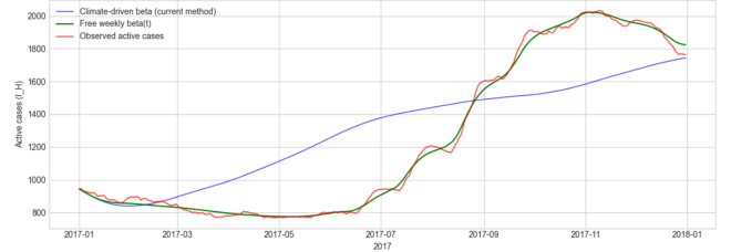
Figure 3: Comparison between the observed active cases and the model estimation of the infectious human compartment I_H for 2017.
