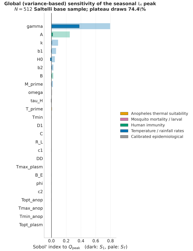
Figure 6: First-order ( S_1 , dark bars) and total-order ( S_T , pale bars) Sobol' indices of the 25 model parameters with respect to the seasonal peak Q_{peak} of the infectious-human compartment, over the whole admissible parameter box of Table 1 (Saltelli design, N = 512 ; bars coloured by parameter group). The total-order index also collects the variance that a parameter carries through its interactions with the remaining ones, hence S_T \geq S_1 . Since Q_{peak} is a maximum, the 74.4% of the sampled parameter sets that are locally subcritical leave it at the initial value I_H(0) ; the indices therefore characterize the sampled box and not the height of an established endemic wave.
