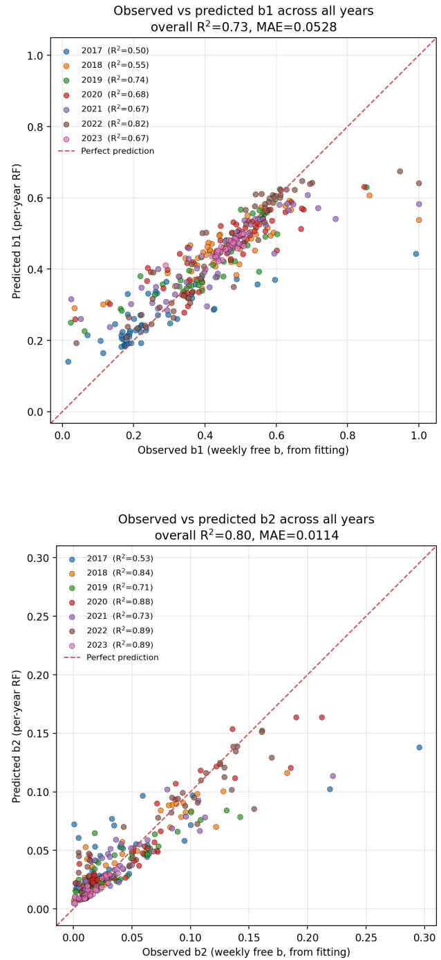
Figure 7: Scatter plot of the estimated vs predicted weekly-free proportion bites from infected humans to susceptible mosquitoes ( b_1 ) and from infected mosquitoes to susceptible humans ( b_2 ) that result in infection.
