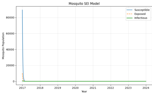
Figure 2A: DDE simulation of the baseline SEI mosquito model using the original parameterization from [7]. The dynamics show that the entire population tended to extinction, an unexpected behavior for a region where malaria is highly endemic.
