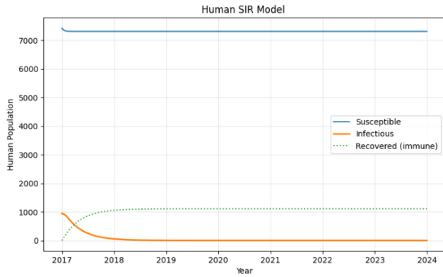
Figure 1A: DDE simulation of the baseline SIR model using the original parameterization from [7]. The dynamics show a monotonic decline in the number of infected individuals, indicating the absence of sustained transmission.
