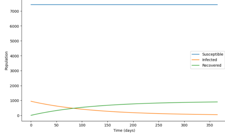
Figure 1A: Simulation of the baseline SIR model using the original parameterization from [? ]. The dynamics show a monotonic decline in the number of infected individuals, indicating the absence of sustained transmission.
