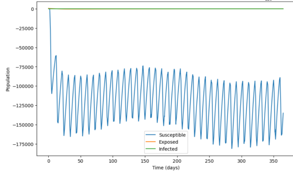
Figure 2A: Simulation of the baseline SEI mosquito model using the original parameterization from [? ]. The susceptible mosquito population exhibits oscillatory behavior and attains negative values, indicating a loss of biological and mathematical consistency.
