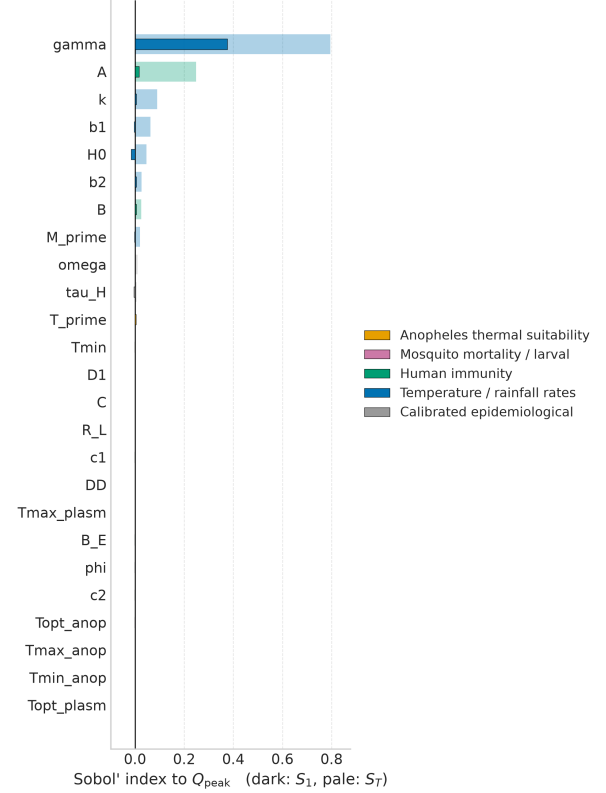
Figure 6: First-order ( S_1 , dark bars) and total-order ( S_T , pale bars) Sobol' indices of the 25 model parameters with respect to the seasonal peak Q_{\text{peak}} of the infectious-human compartment, over the whole admissible parameter box of Table 1 (Saltelli design, N = 512 ; bars coloured by parameter group). The total-order index also collects the variance that a parameter carries through its interactions with the remaining ones, hence S_T \geq S_1 . Since Q_{\text{peak}} is a maximum, the 74.4% of the sampled parameter sets that are locally subcritical leave it at the initial value I_H(0) ; the indices therefore characterize the sampled box and not the height of an established endemic wave.
