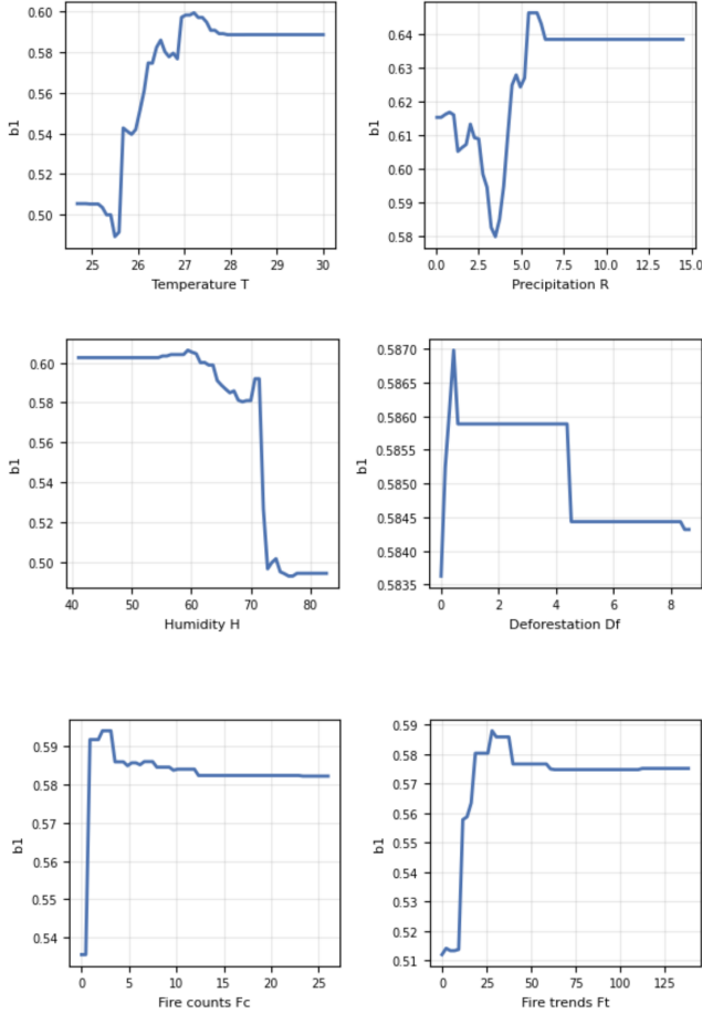
Figure 8: Partial dependence of the weekly per-bite transmission probability b_1 on each environmental predictor in 2022.
