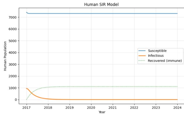
Figure 1A: DDE simulation of the baseline SIR model using the original parameterization from Parham & Michael (2010) [7]. The dynamics show a monotonic decline in the number of infected individuals, indicating the absence of sustained transmission.
