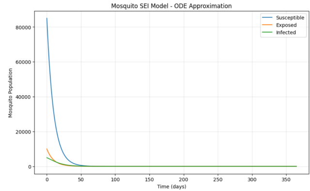
Figure 4A: ODE simulation of the baseline SEI mosquito model using the formulation from 2.2 and parameters from [7]. It can be seen that the mosquito population still tends to extinction.
