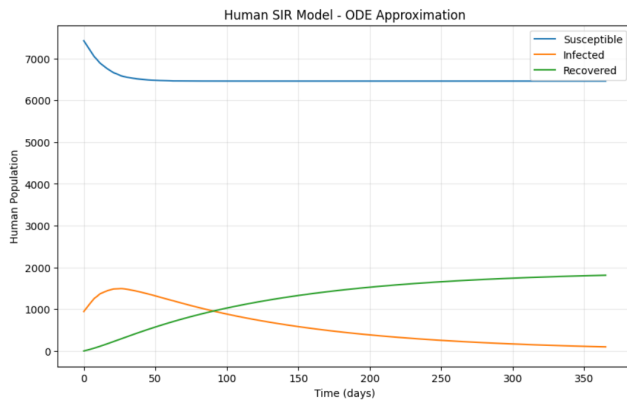
Figure 3A: ODE simulation of the baseline SIR model using the formulation from 2.2 and parameters from [7].
