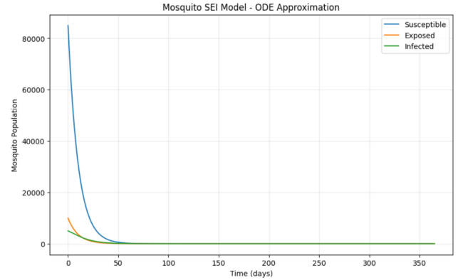
Figure 4A: ODE simulation of the baseline SEI mosquito model using the formulation from 2.2 and parameters from [7].
