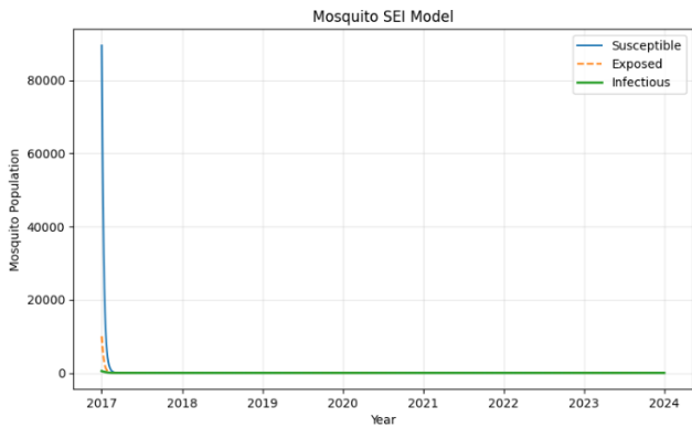
Figure 2A: DDE simulation of the baseline SEI mosquito model using the original parameterization from [7]. The dynamics show that the entire population tended to extinction, an unexpected behavior for a region where malaria is highly endemic.
