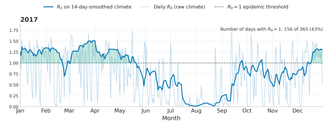
Figure 4: Seasonal variation of the basic reproduction number R_0 for the calibrated model in 2017.
