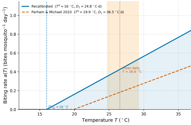
Figure 2: Comparison between the recalibrated temperature-dependent biting rate a(T) used in this work ( T' = 16^\circ\text{C} , D_1 = 24.8^\circ\text{Cdays} ) and the original Parham & Michael (2010) parameterization [11] ( T' = 19.9^\circ\text{C} , D_1 = 36.5^\circ\text{Cdays} ). The shaded band indicates the range of daily mean temperatures observed in Manaus between 2017 and 2023 (5th-95th percentiles), and the dashed vertical line marks the recalibrated biting threshold T' = 16^\circ\text{C} .
