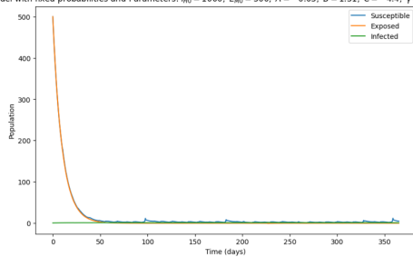
Figure 3A: Simulation of the SEI mosquito model after modifying parameter functions to enforce biologically admissible bounds on probabilities and rates. Although positivity is restored, the mosquito population rapidly declines toward extinction, suggesting that additional mechanisms are required to sustain endemic transmission.
