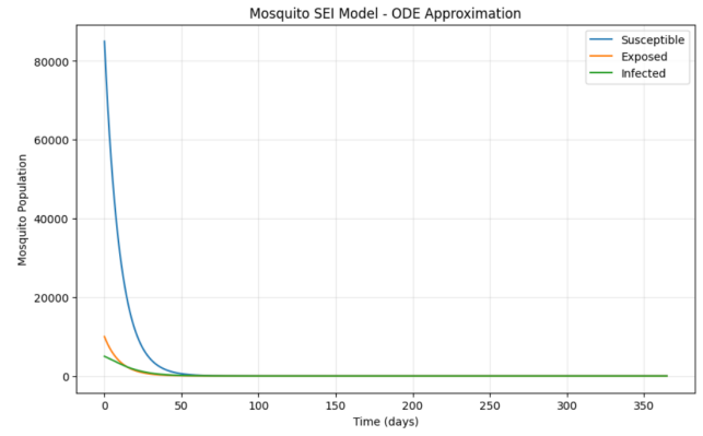
Figure 3A: ODE simulation of the baseline SEI mosquito model using the formulation from Section 2.2 and parameters from [11]. It can be seen that the mosquito population still tends to extinction.
