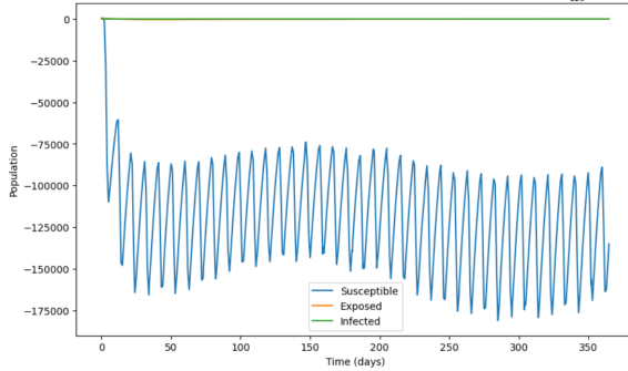
Figure 2A: Simulation of the baseline SEI mosquito model using the original parameterization from [? ]. The susceptible mosquito population exhibits oscillatory behavior and attains negative values, indicating a loss of biological and mathematical consistency.
