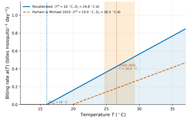
Figure 1: Comparison between the recalibrated temperature-dependent biting rate a(T) used in this work ( T' = 16^\circ\text{C} , D_1 = 24.8^\circ\text{C days} ) and the original Parham & Michael (2010) parameterization [18] ( T' = 19.9^\circ\text{C} , D_1 = 36.5^\circ\text{C days} ). The shaded band indicates the range of daily mean temperatures observed in Manaus between 2017 and 2023 (5th–95th percentiles), and the dashed vertical line marks the recalibrated biting threshold T' = 16^\circ\text{C} .
