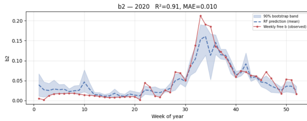
Figure 2: Best within-year random-forest fit of the freed weekly per-bite transmission b_1 and b_2 , in 2022 and 2020 respectively.
