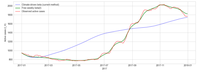
Figure 1: Comparison between the observed active cases and the model estimation of the infectious human compartment I_H for 2017.
