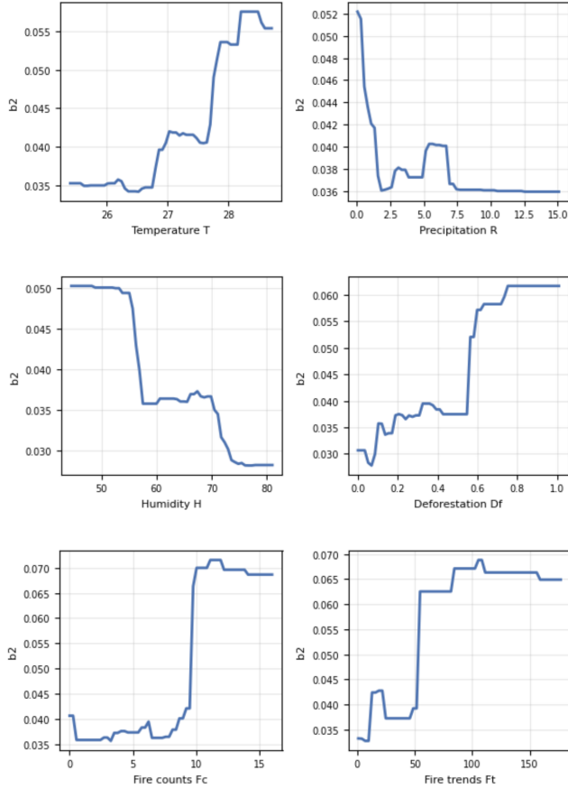
Figure 4: Partial dependence of the weekly per-bite transmission probability b_2 on each environmental predictor in 2020.
