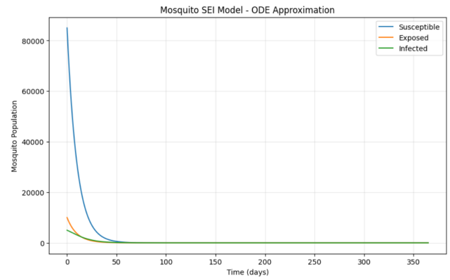
Figure 3A: ODE simulation of the baseline SEI mosquito model using the formulation from Section 3.2 and parameters from [18]. It can be seen that the mosquito population still tends to extinction.
