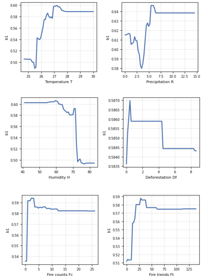
Figure 2: Best within-year random-forest fit of the freed weekly per-bite transmission b_1 and b_2 , in 2022 and 2020 respectively.
