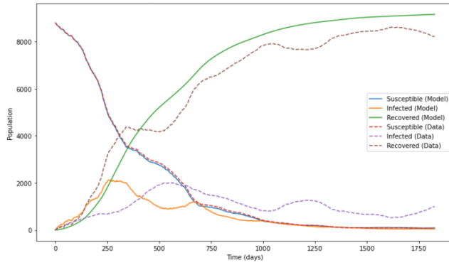
Figure 1A: Ex.: Comparison between observed data of infections and model estimation of I_H .
