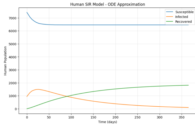
Figure 2A: ODE simulation of the baseline SIR model using the formulation from Section 3.2 and parameters from [16]. A slight increase in the infectious population can be noticed, although it still tends to extinction over the course of the first year of transmission.
