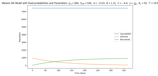
Figure 1A: Simulation of the baseline SIR model using the original parameterization from [7]. The dynamics show a monotonic decline in the number of infected individuals, indicating the absence of sustained transmission.
