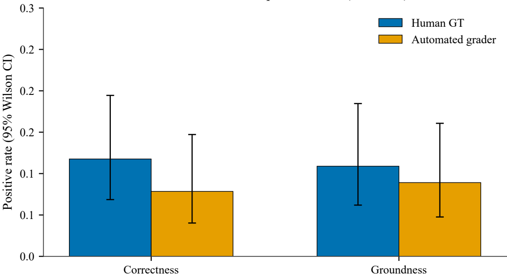
Human vs automated positive rates (strictness)
