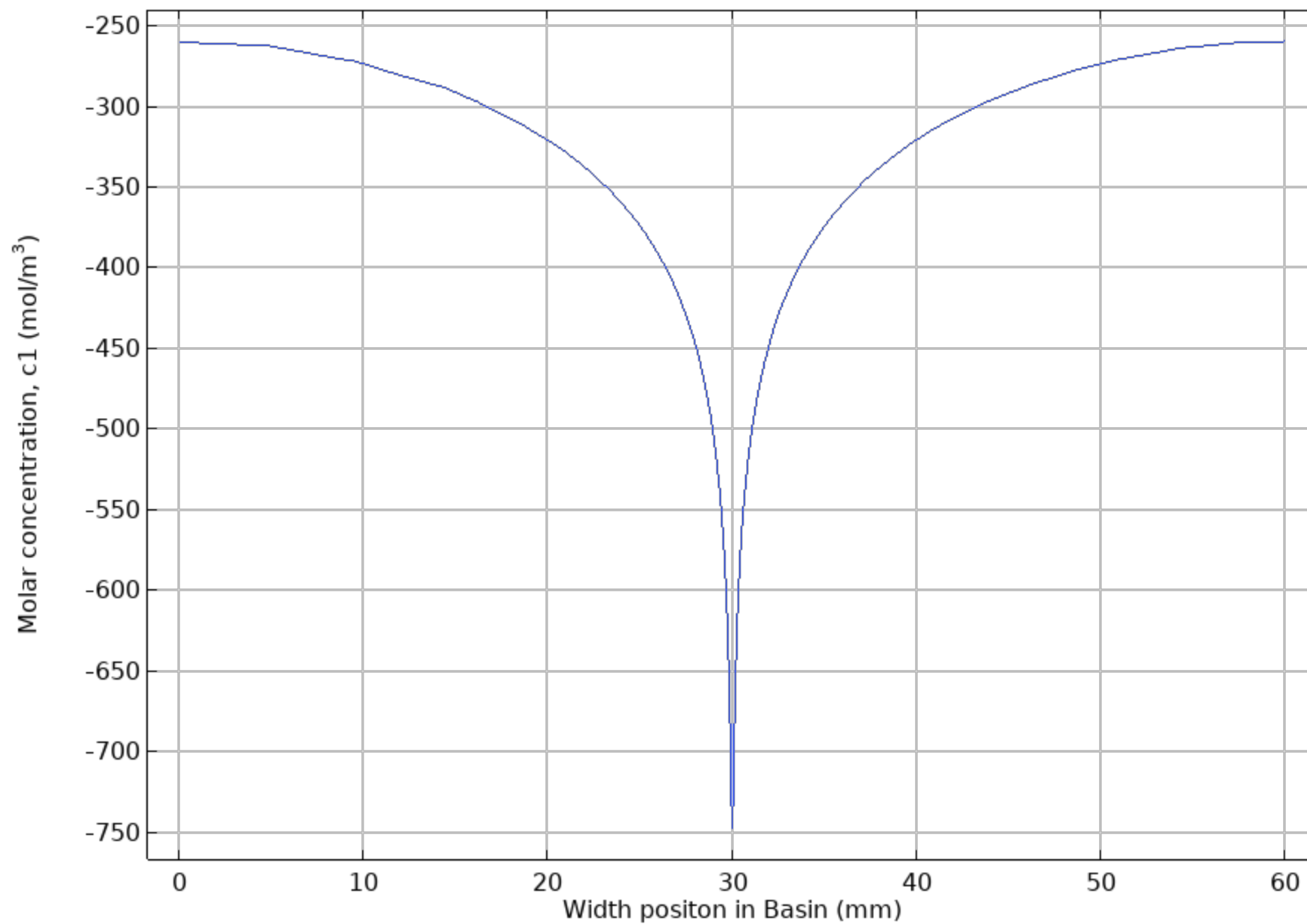
Molar concentration, Ni ( \text{mol/m}^3 ), measured horizontally cut across wire
