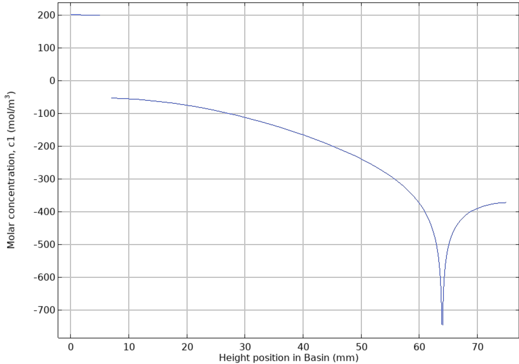
Molar concentration, Ni ( \text{mol/m}^3 ), measured vertically cut across wire
