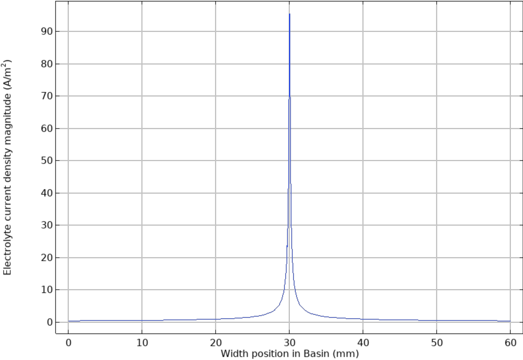
Comparison of current density line graphs: Different planes measured horizontally across the wire (A/m 2 )
