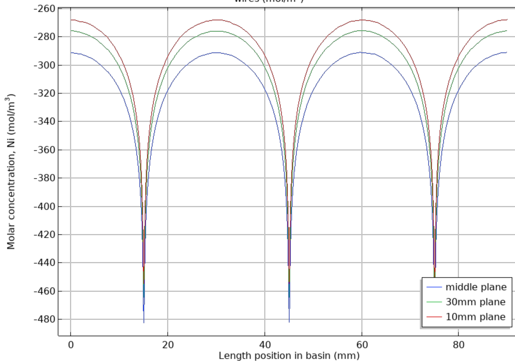
Comparison of ion concentration line graphs: Different planes measured horizontally across the wires (mol/m 3 )
