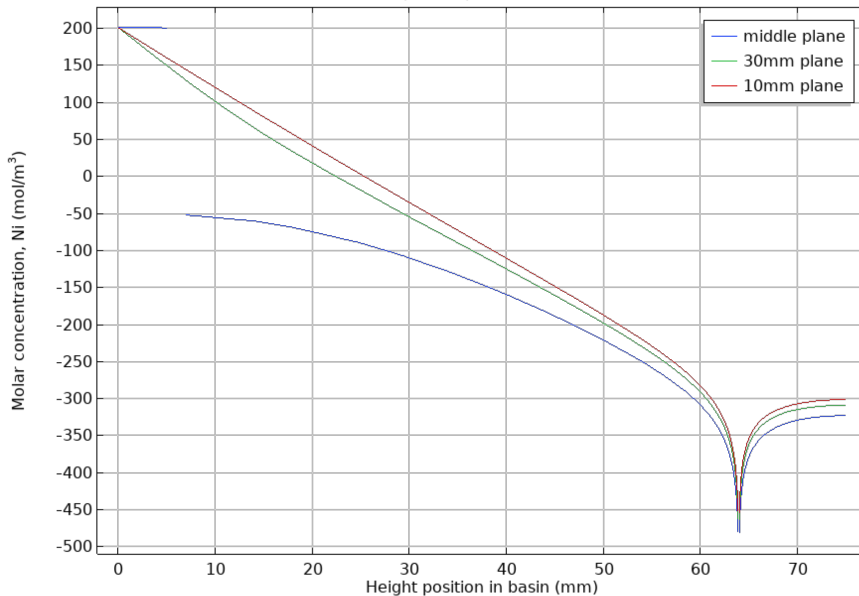
Comparison of ion concentration line graphs: Different planes measured vertically across the wires (mol/m 3 )
