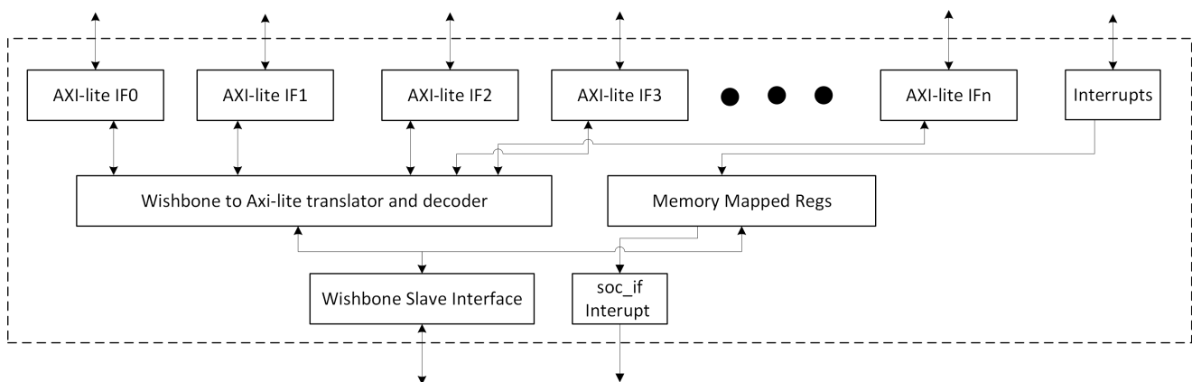
Figure 7. SoC interface
