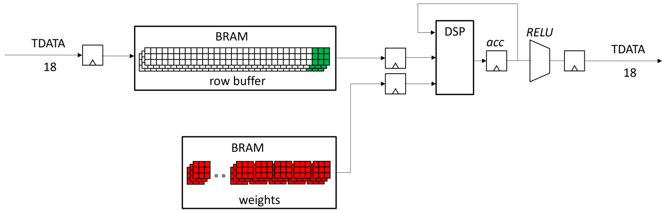
Figure 5. System Diagram
