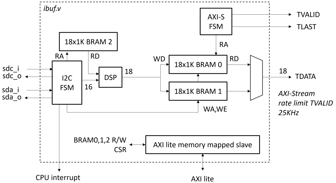
Figure 3. Input buffer
