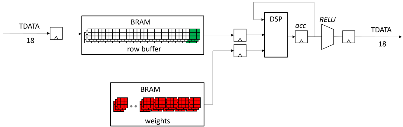
Figure 5. System Diagram
