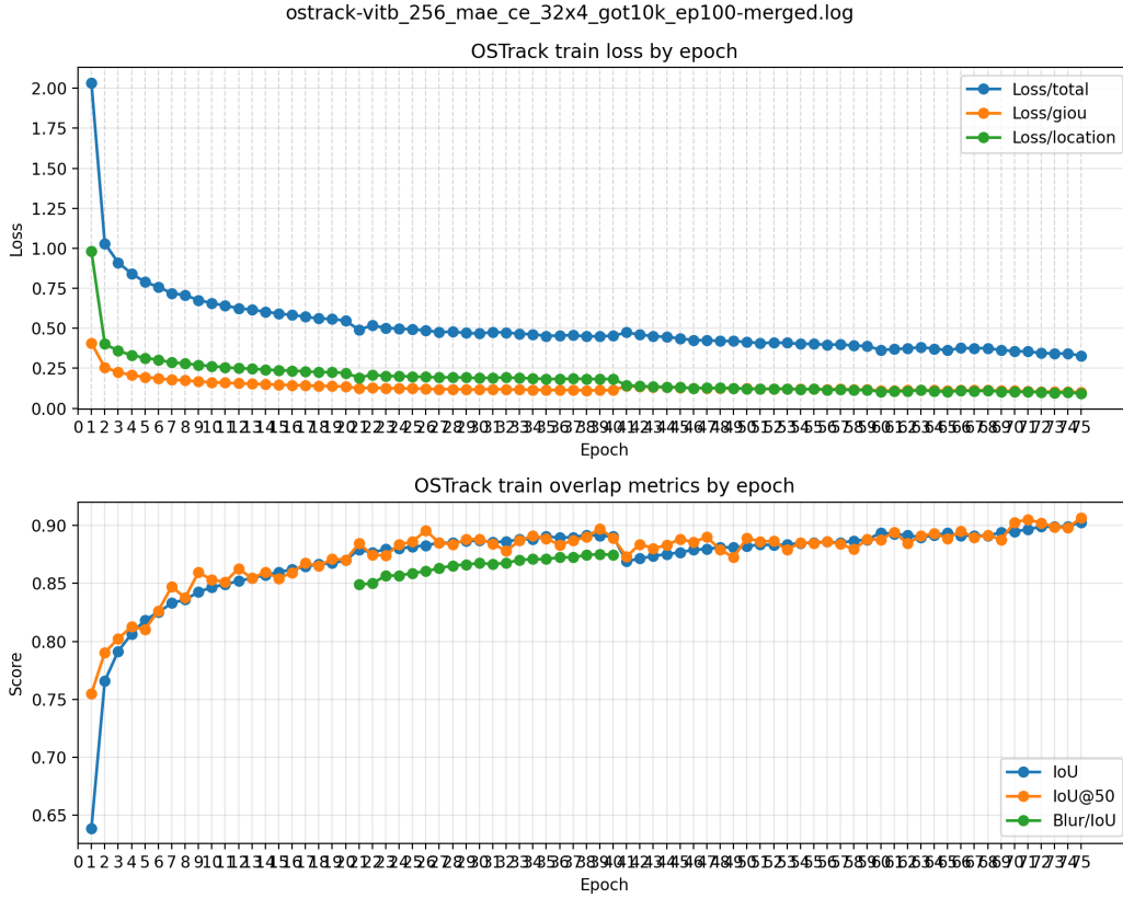
Figure 7.1: Training loss and overlap metrics over the 75 recorded epochs, illustrating the impact of the different training phases.
