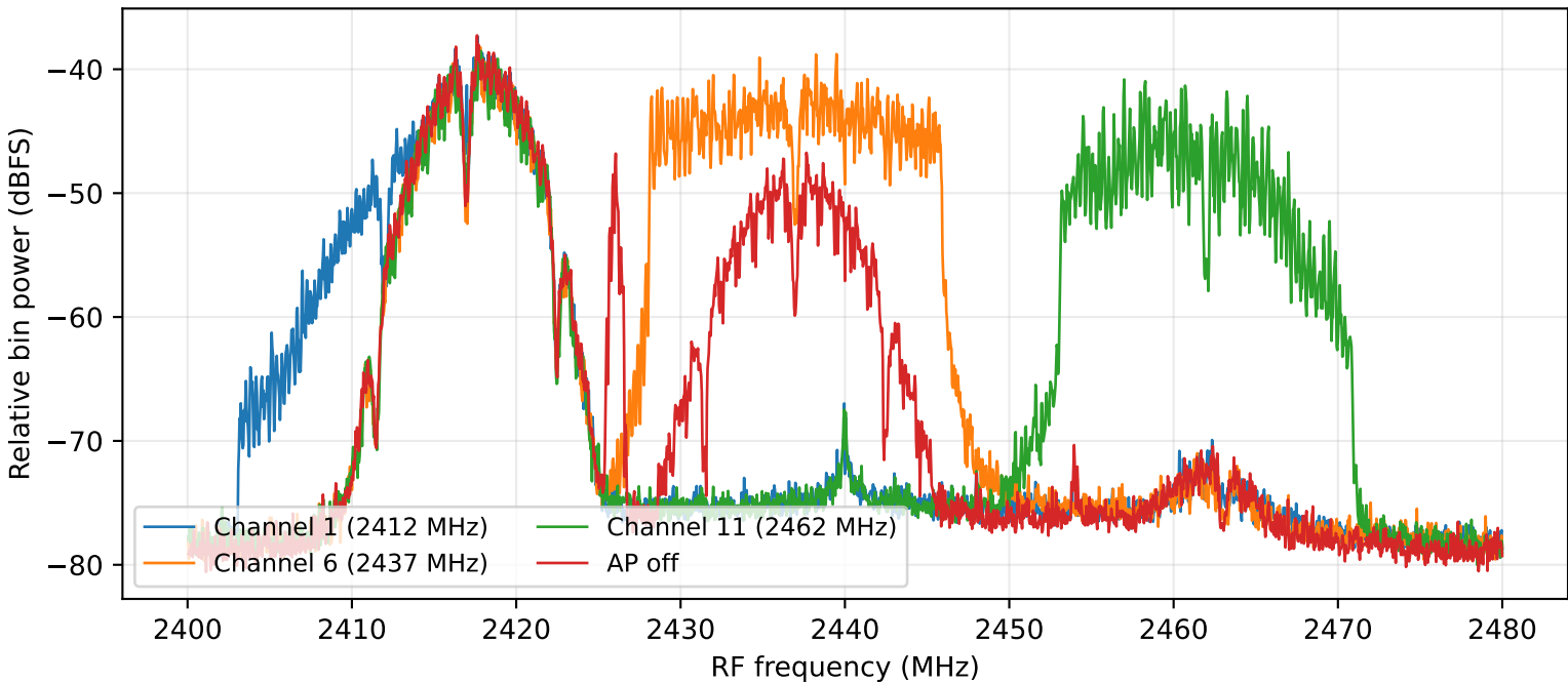
Channel selection under requested 20 Mbps downlink
