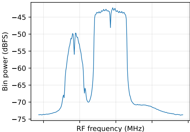
N=1024, bin spacing=78.12 kHz
