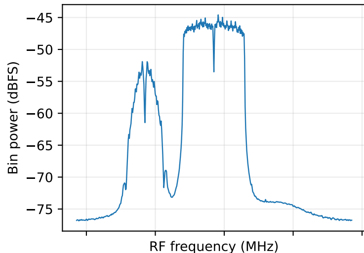
N=2048, bin spacing=39.06 kHz
