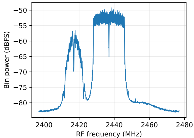
N=2048, bin spacing=39.06 kHz
