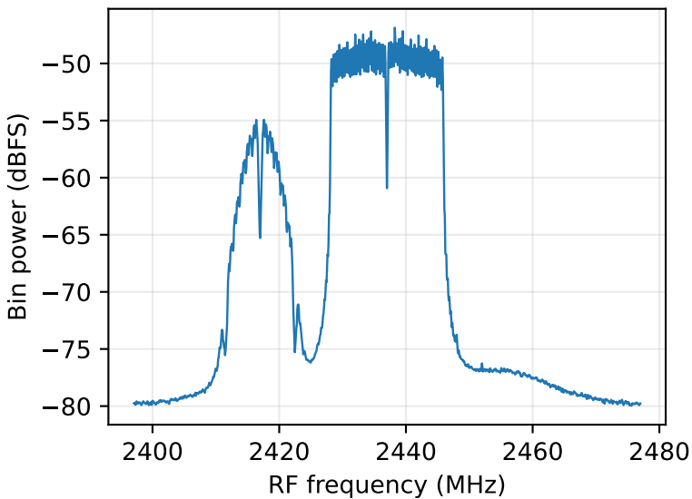
N=1024, bin spacing=78.12 kHz
