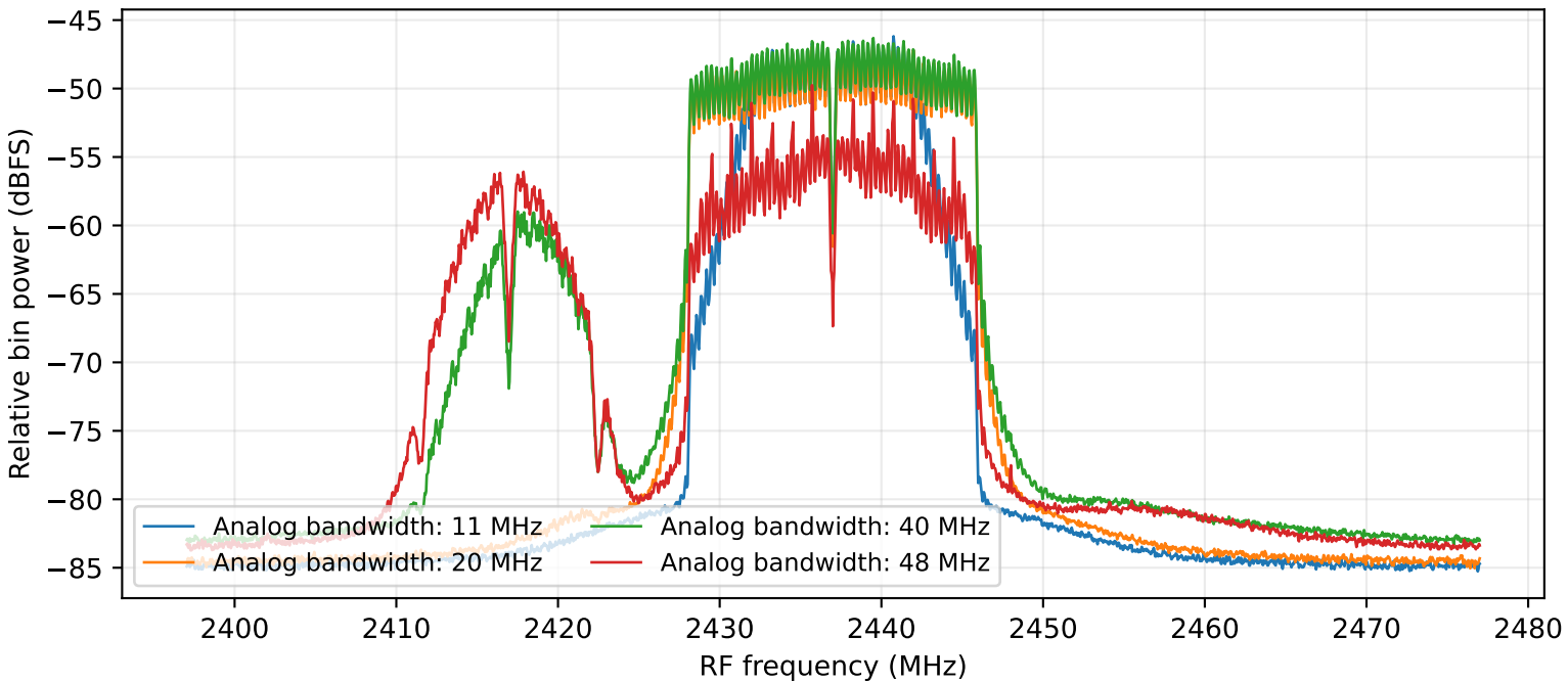
Analog receive bandwidth, requested 20 Mbps downlink
