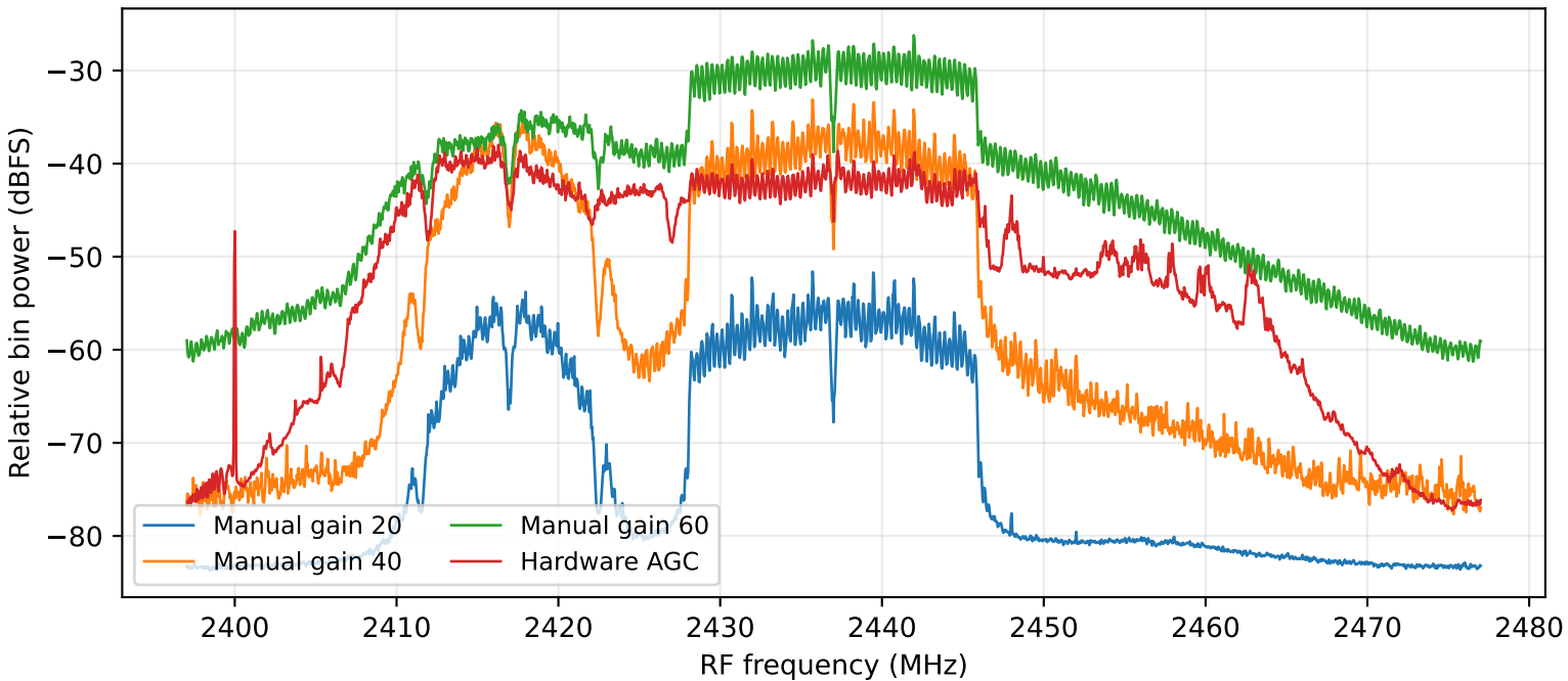
Receiver gain affects signal, noise and saturation
