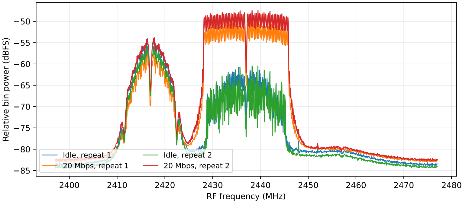
Idle versus loaded AP, channel 6
