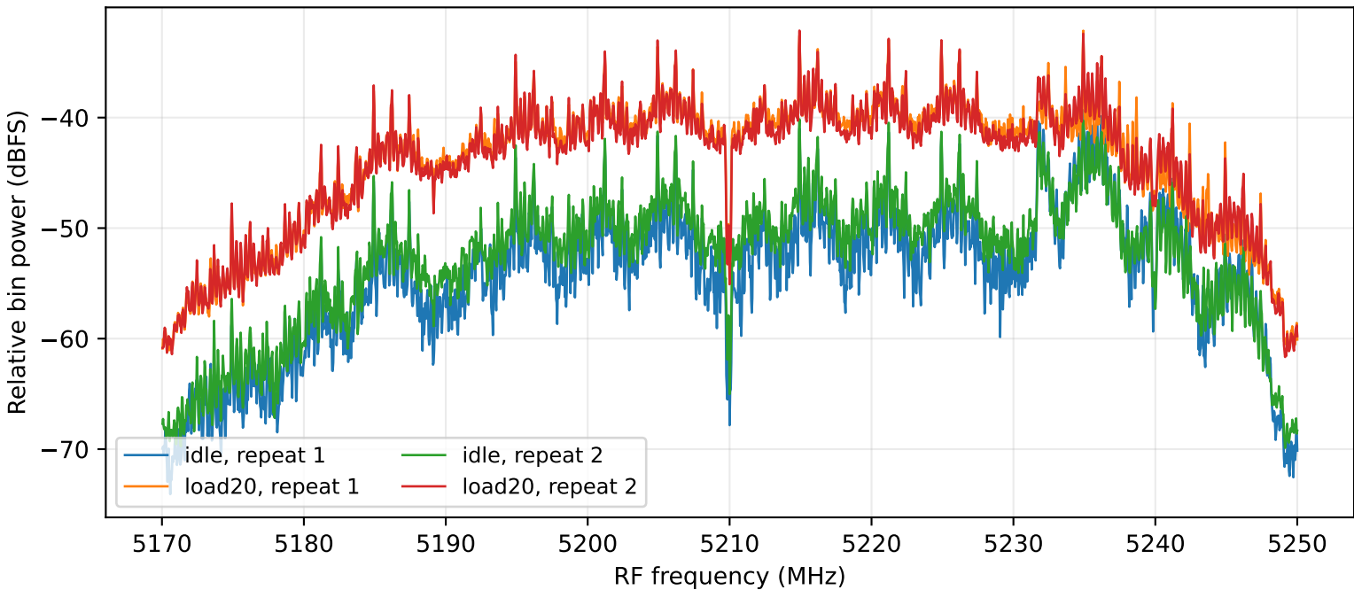
Existing 5 GHz router: primary 5240 MHz, center 5210 MHz
