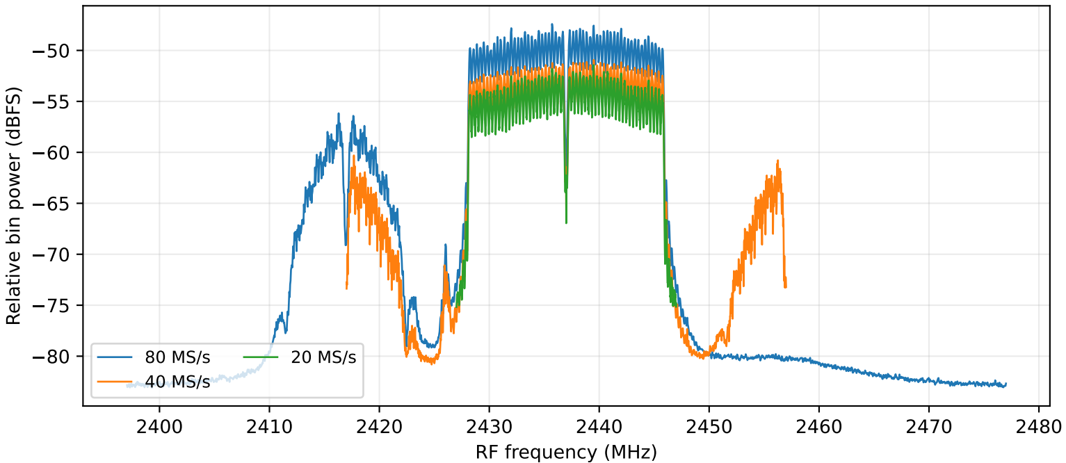
Sample rate changes the observed span and bin spacing
