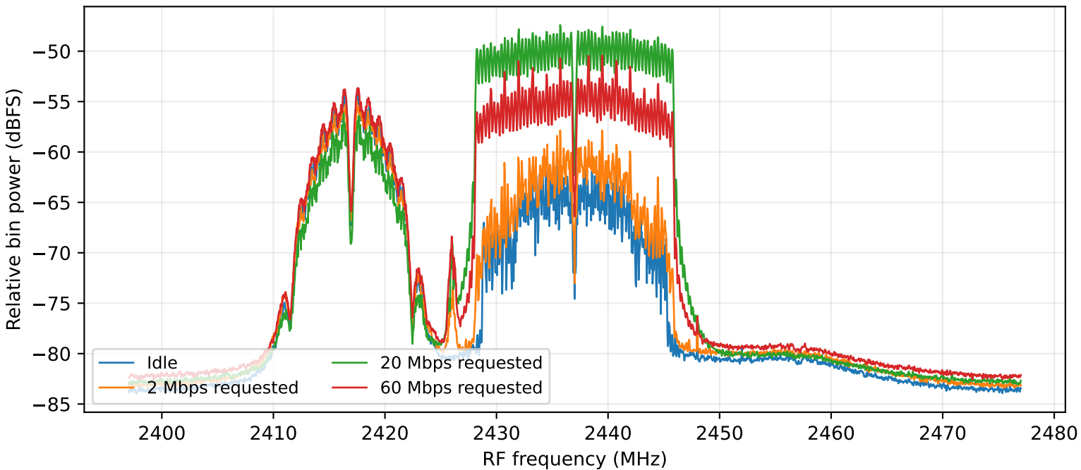
TCP traffic demand and measured spectrum, channel 6
