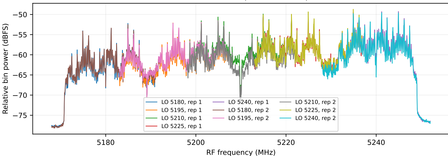
Overlap-weighted 80 MHz reconstruction; no amplitude calibration
