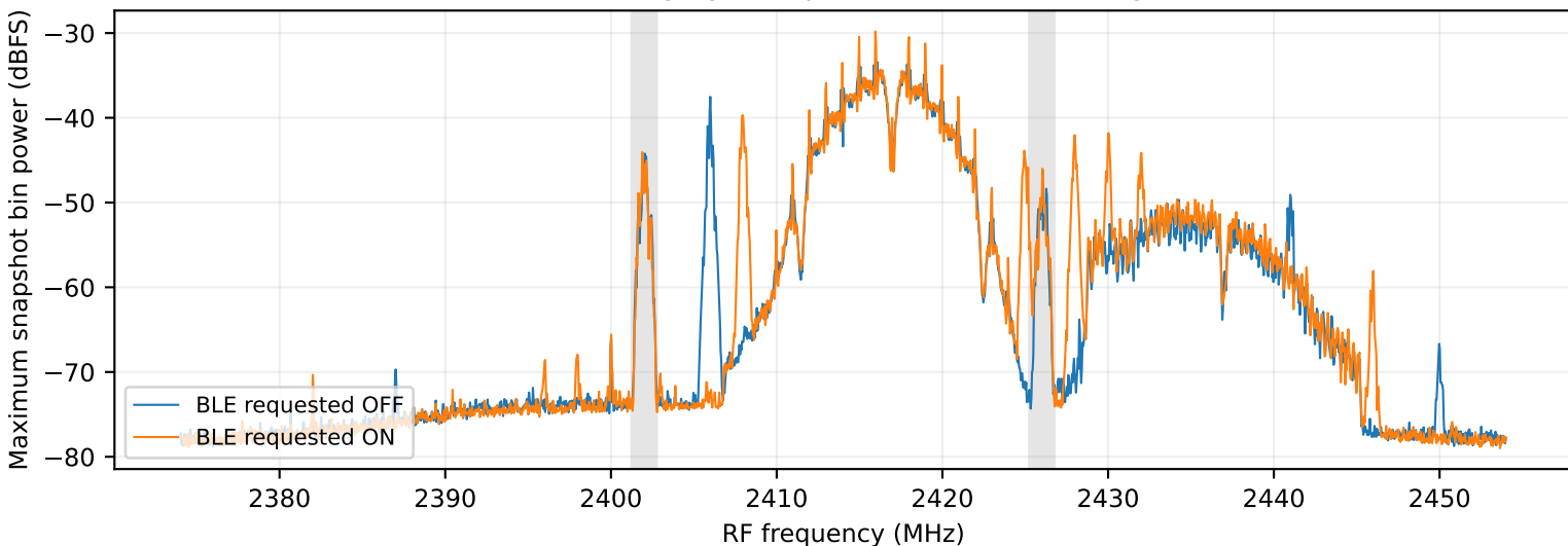
LO 2475 MHz; grey = expected BLE advertising bands
