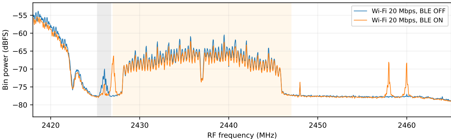
Maximum of actual snapshots; grey = 2426 MHz advertising band
