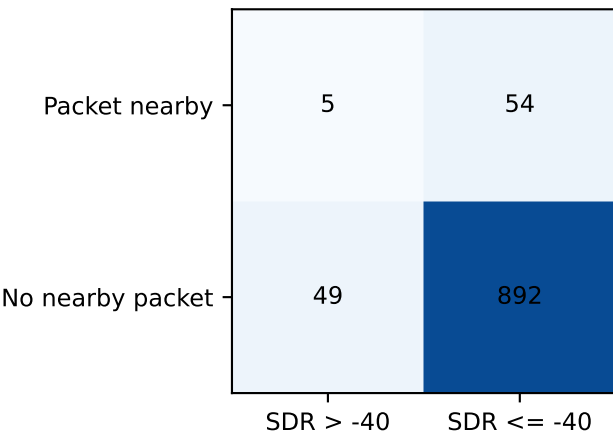
pcap-idle, extra +/-20 ms
