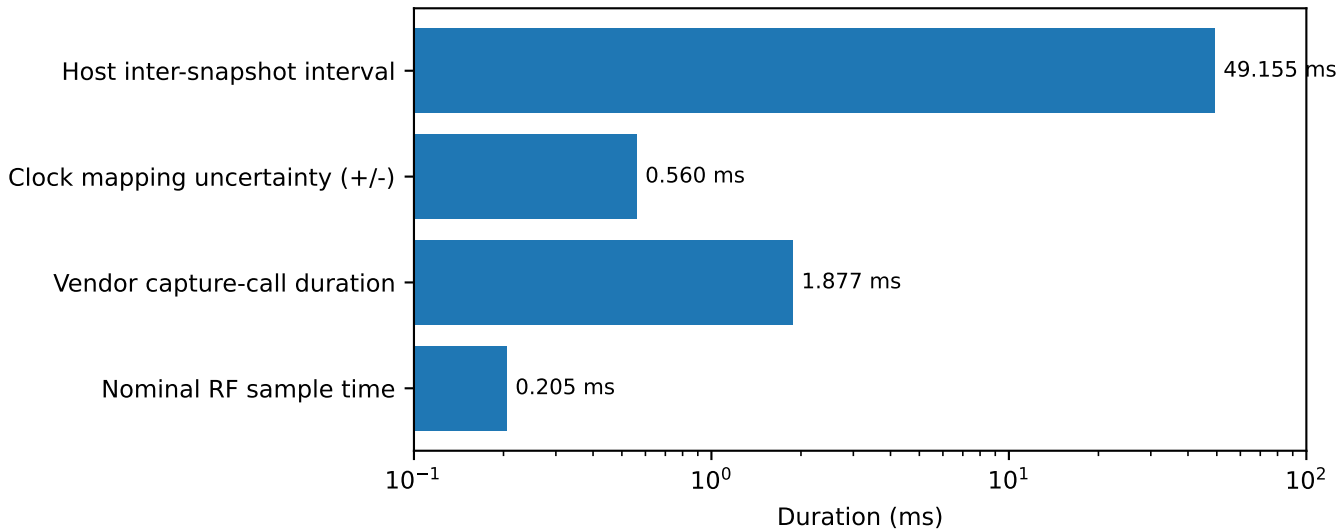
Four different time scales (80 MS/s)
