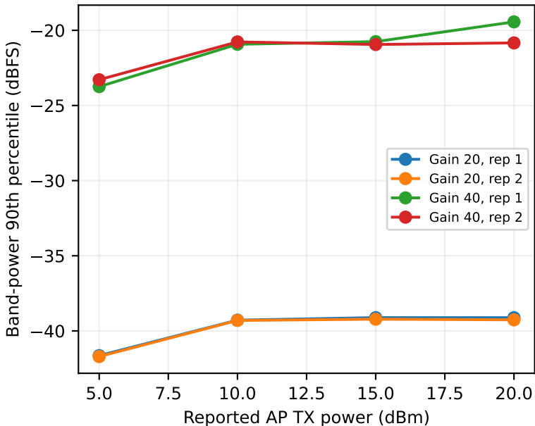
Over-the-air power-setting response
