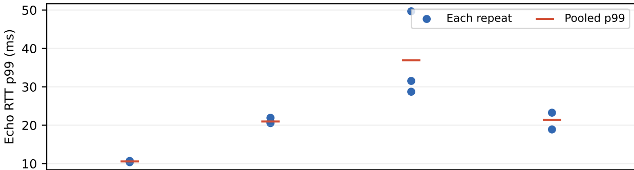
100 Hz UDP echo to ESP32; same AP TCP downlink
