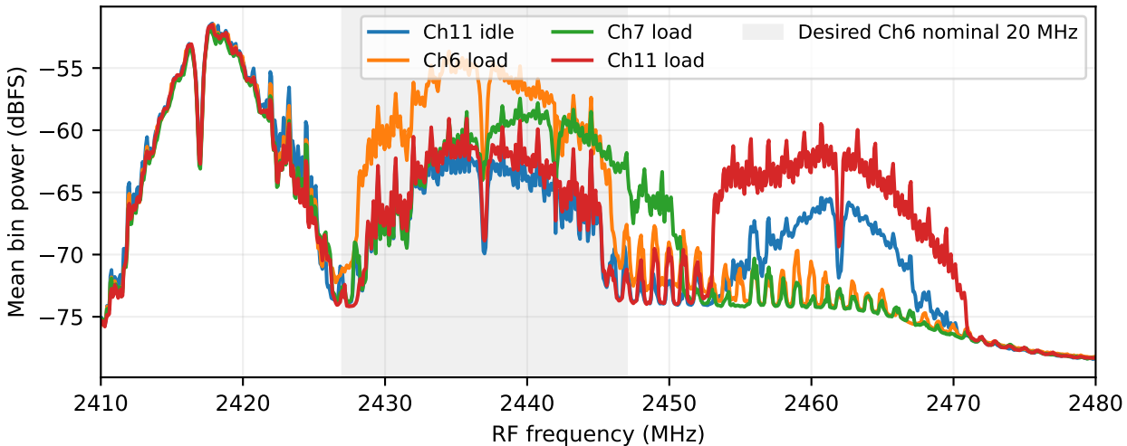
Measured spectra at fixed LO=2442 MHz, gain 20
