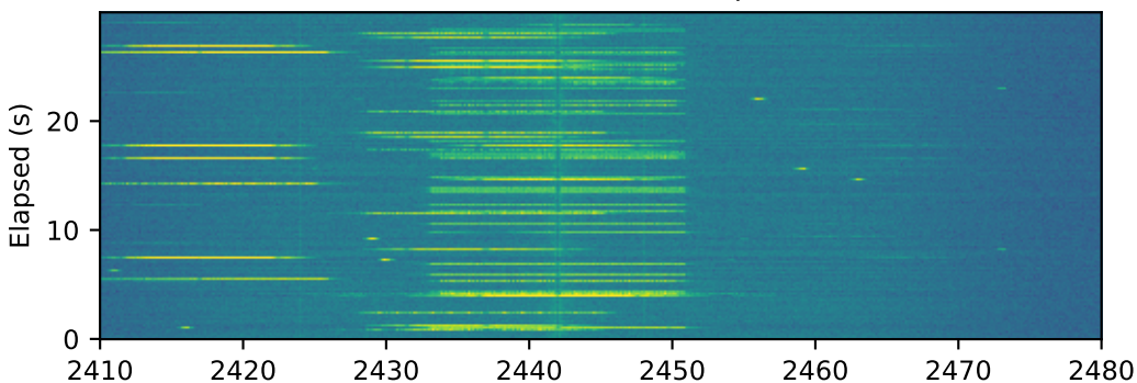
Ch11; intermittent I/Q snapshots
