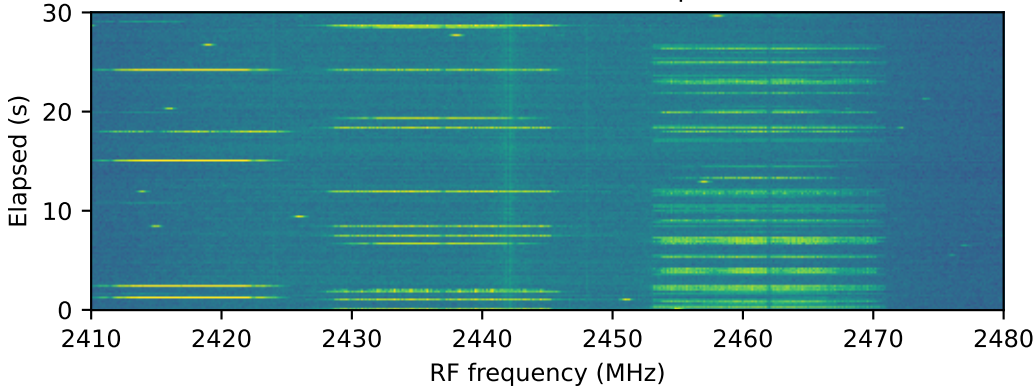
Ch11; intermittent I/Q snapshots
